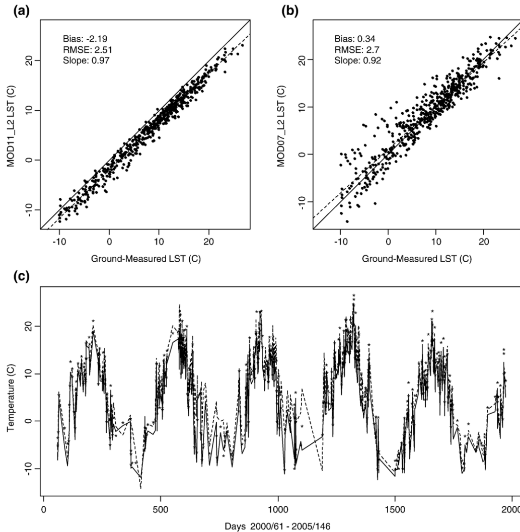
Fig. 5. Plots for Fort Peck grassland site (a) ground-measured LSTs vs. MOD11_L2 LSTs (b) ground-measured LSTs vs. MOD07_L2 LSTs (c) time series of MOD11_L2 LSTs (solid line), MOD07_L2 LSTs (dash line), and ground-measured LSTs (*).
