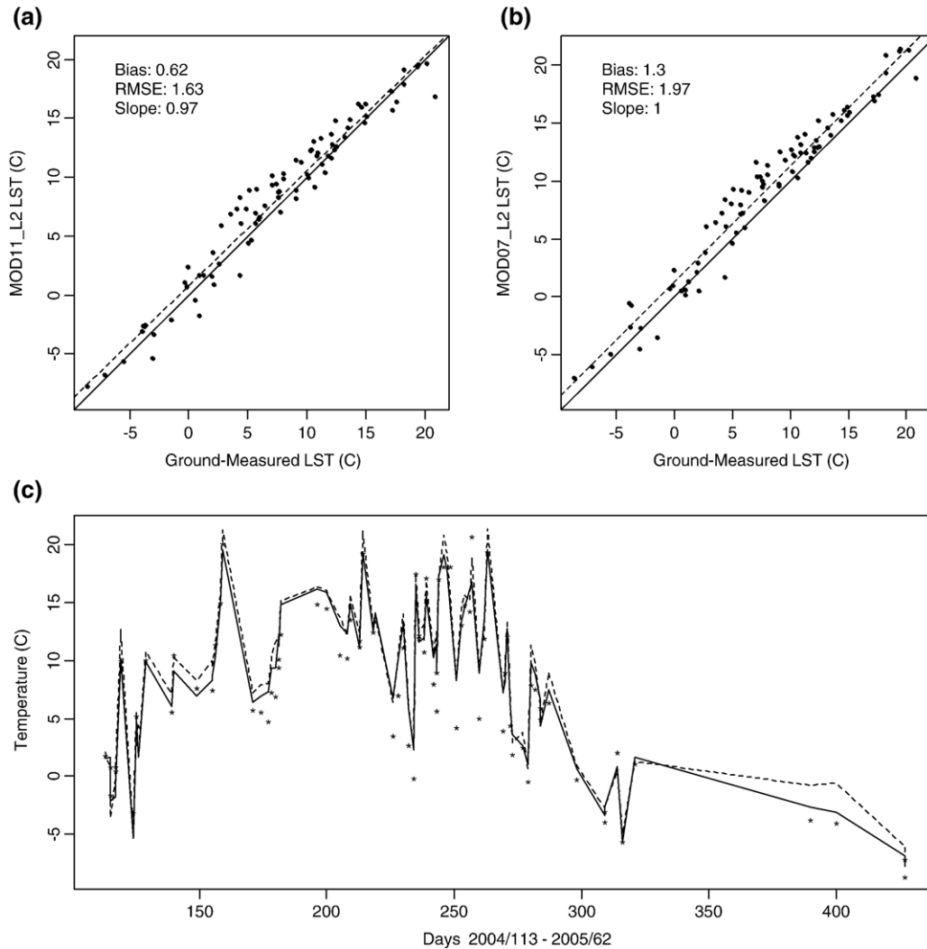
Fig. 1. Plots for Brookings grassland site (a) ground-measured LSTs vs. MOD11_L2 LSTs (b) ground-measured LSTs vs. MOD07_L2 LSTs (c) time series of MOD11_L2 LSTs (solid line), MOD07_L2 LSTs (dash line), and ground-measured LSTs (*).
