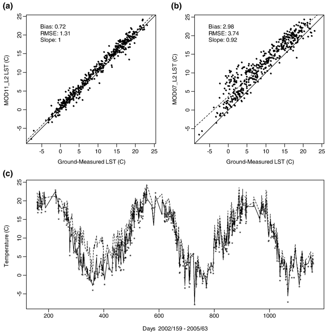
Fig. 2. Plots for Audubon grassland site (a) ground-measured LSTs vs. MOD11_L2 LSTs (b) ground-measured LSTs vs. MOD07_L2 LSTs (c) time series of MOD11_L2 LSTs (solid line), MOD07_L2 LSTs (dash line), and ground-measured LSTs (*).
